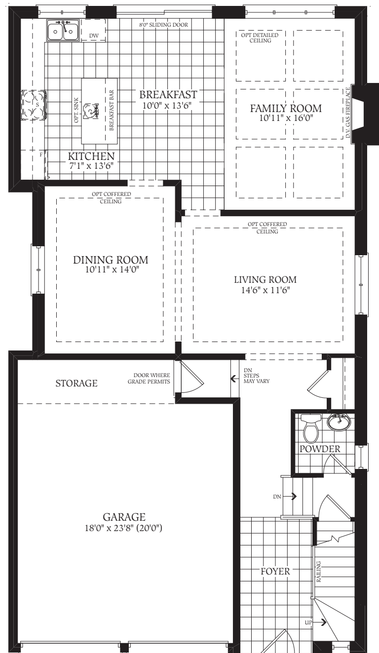
GROUND FLOOR ELEVATION B
