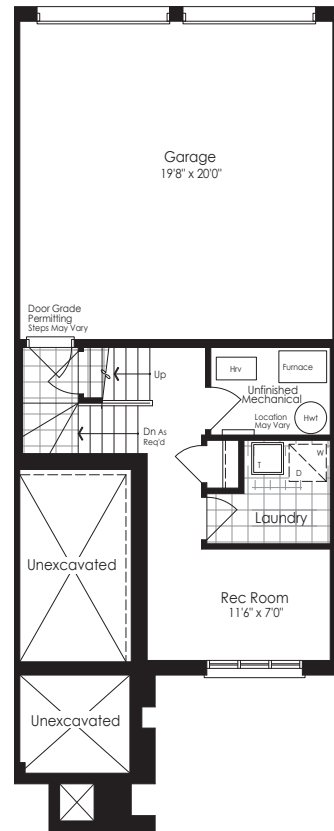
ALT. GROUND FLOOR Elevation A & B
