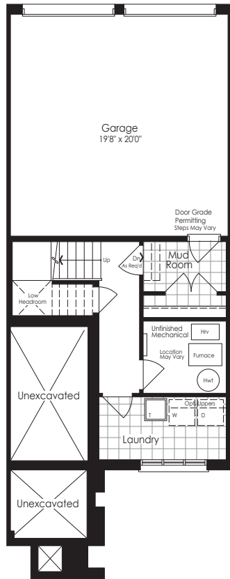
GROUND FLOOR Elevation A & B
