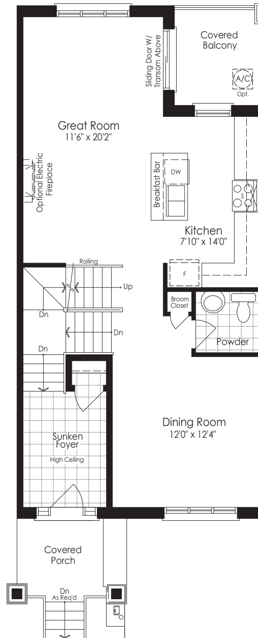
MAIN FLOOR Elevation A & B
